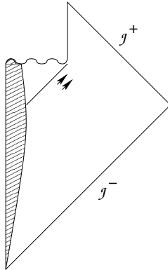
FIG. 2. The standard space-time diagram depicting black hole evaporation
