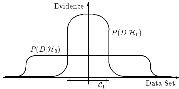
Figure 2: Why Bayes embodies Occam’s razor
