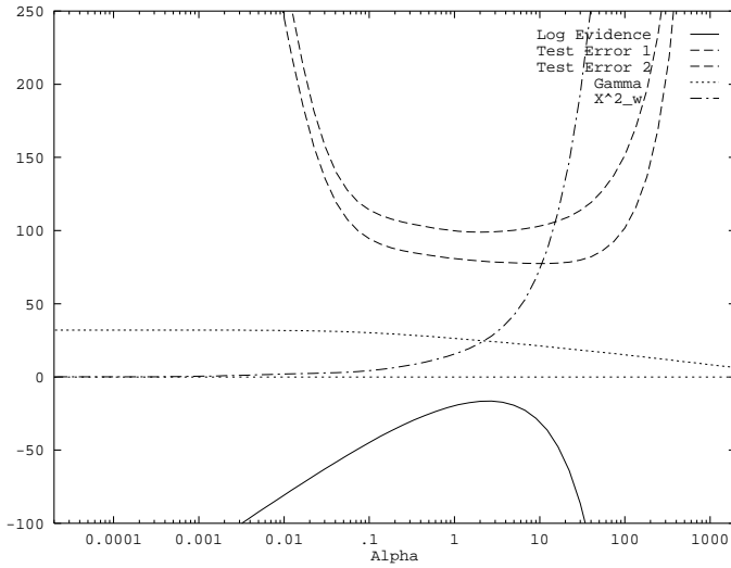
Figure 5: Choosing \alpha
