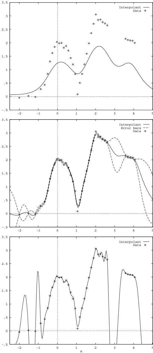
Figure 4: How the best interpolant depends on \alpha
