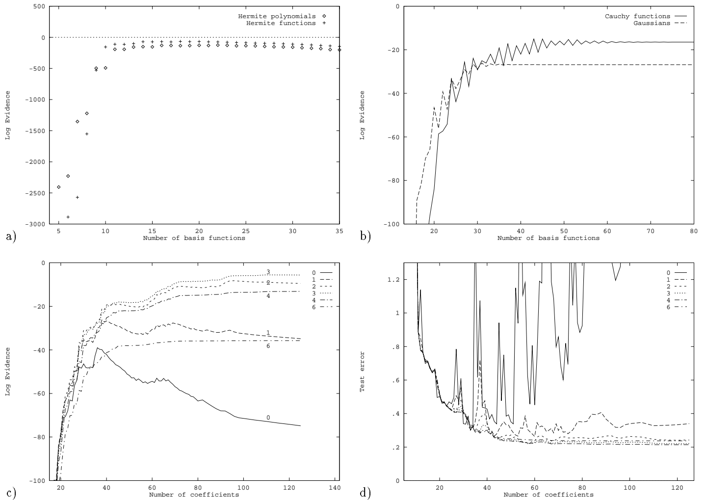
Figure 7: The Evidence for data set X
