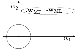
Figure 6: Good and bad parameter measurements w_1 and w_2 are the components in parameter space in two directions parallel to eigenvectors of the data matrix \mathbf{B} . The circle represents the characteristic prior distribution for \mathbf{w} . The ellipse represents a characteristic contour of the likelihood, centred on the maximum likelihood solution \mathbf{w}_{ML} . \mathbf{w}_{MP} represents the most probable parameter vector. w_1 is a direction in which \lambda_1 is small compared to \alpha , i.e. the data have no strong preference about the value of w_1 ; w_1 is a poorly measured parameter, and the term \frac{\lambda_1}{\lambda_1 + \alpha} is close to zero. w_2 is a direction in which \lambda_1 is large; w_2 is well determined by the data, and the term \frac{\lambda_2}{\lambda_2 + \alpha} is close to one.
